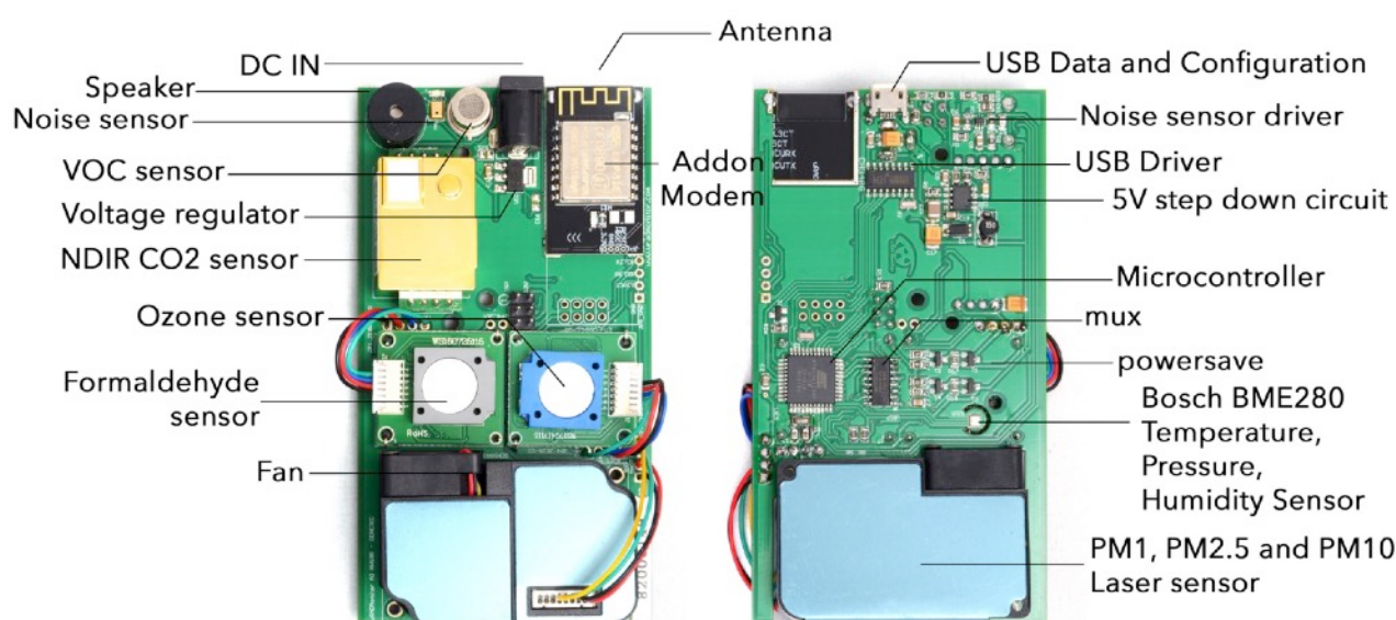
uRADMonitor Model A3
