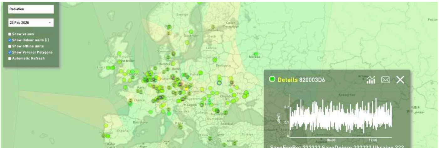
Figure 5: Voronoi view
